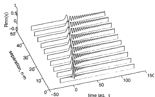
Figure 5: Cross correlation, R_{m,n}(\tau) , between the m th and the n th capacitor voltages in the linearized line.
