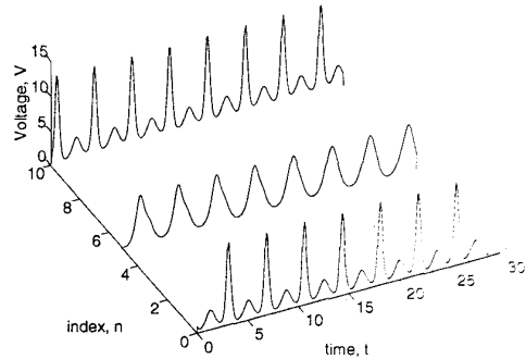
Figure 3: Soliton modulation of Suzuki et al.
