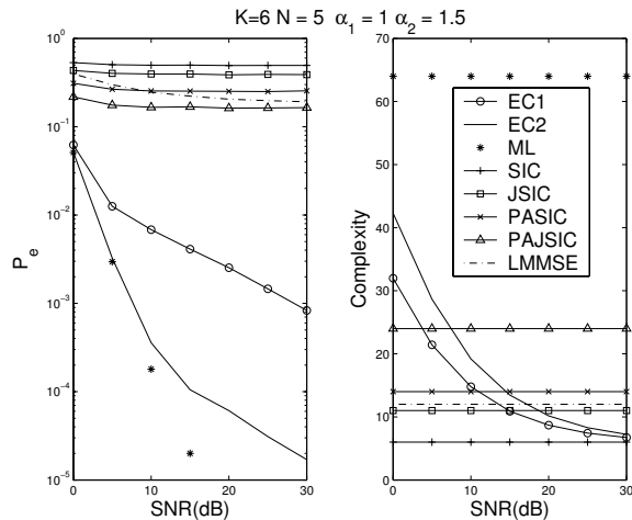
(a) P_e and detection complexity plotted against SNR
