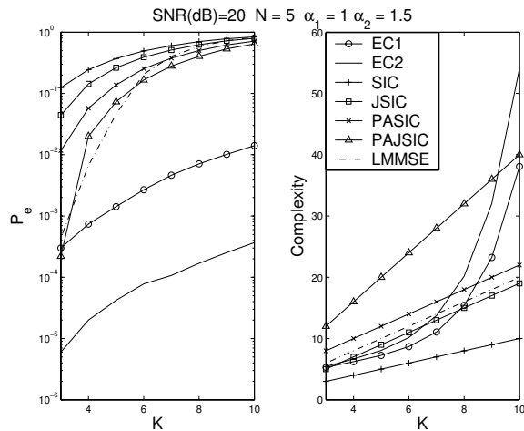
(b) P_e and detection complexity plotted against K
