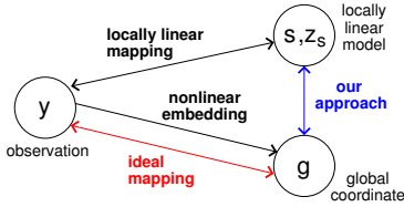
Figure 2: Mappings of nonlinear dimensionality reduction schemes.
