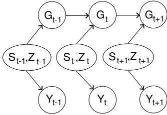
Figure 4: Our generative model for dynamic textures.
