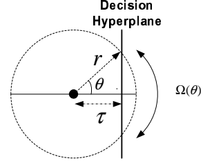
Fig. 2. Decision boundary \tau and norm r of noise vector \mathbf{E} .
