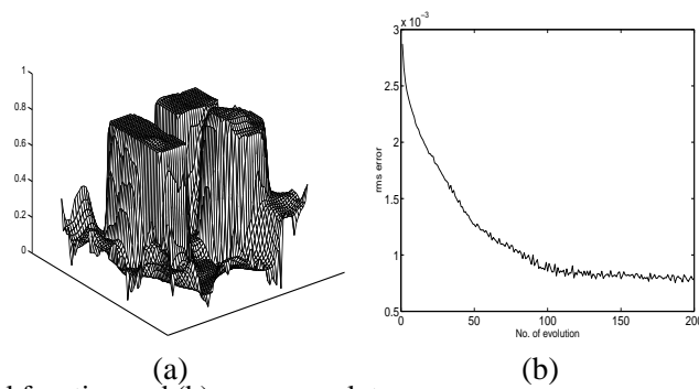
Figure 6. Example 2: (a) level function and (b) rms error plot
