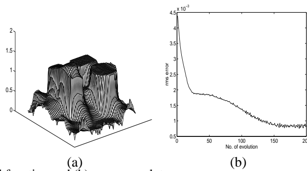
Figure 4. Example 1 (a) level function and (b) rms error plot
