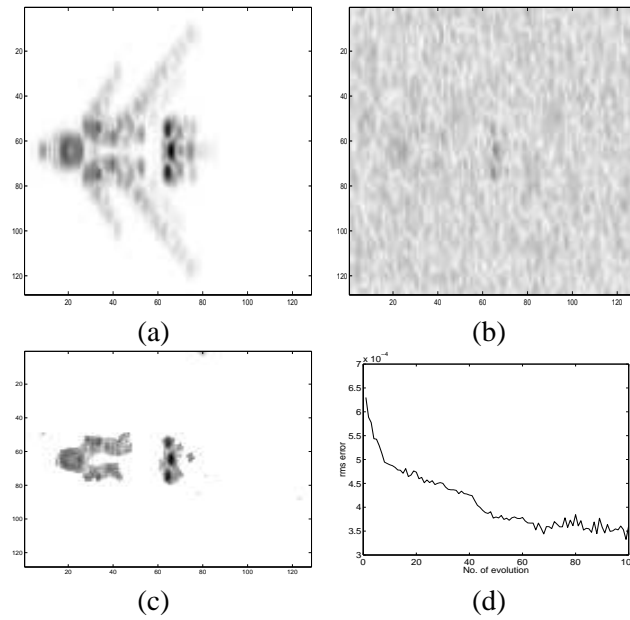
Figure 8. Example 3: (a) original VFY aircraft image, (b) direct Fourier reconstruction, (c) reconstruction by our algorithm, and (d) rms error plot.
