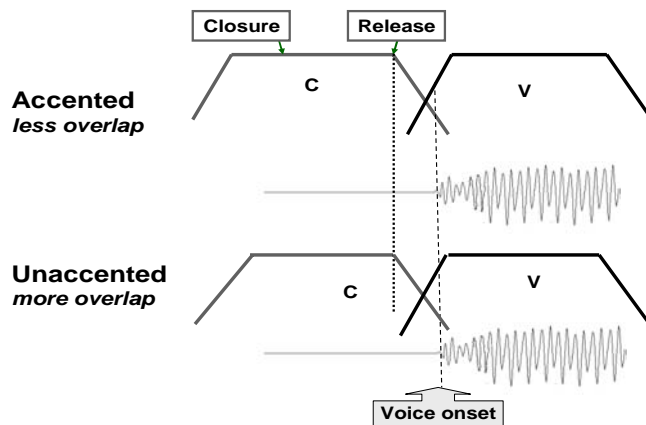
Figure 2a. Schematic diagram of C and V gestures showing less inter-gestural overlap in the Accented condition (top) than in the Unaccented condition (bottom). The locus-equation F2-onset measure is taken at the location marked by voice onset.
